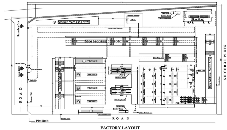
FACTORY LAYOUT
